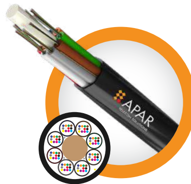
Loose Tube Microduct Cable Range: 12F-288F
